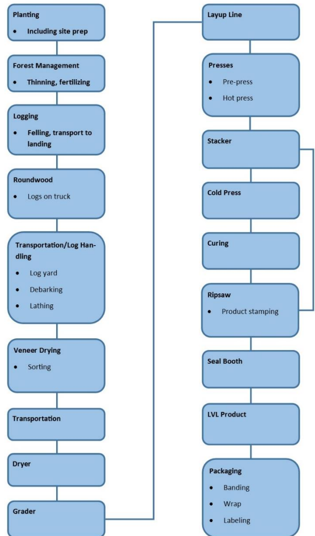
Figure 1: Cradle-to-gate product system for laminated veneer lumber
