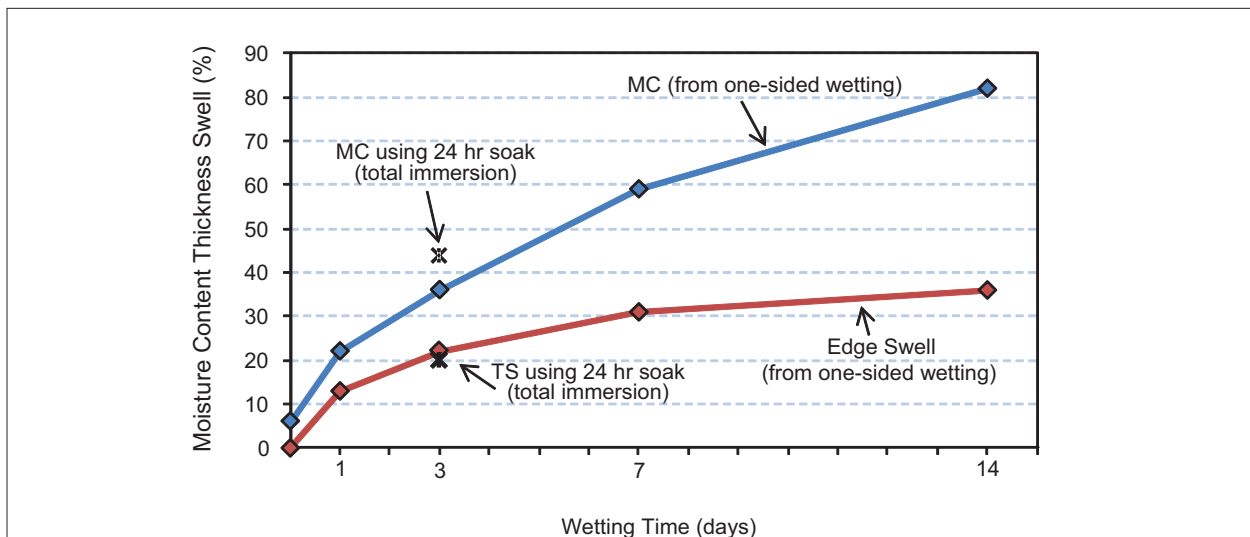
Figure 3. OSB Sheathing Response to One-Sided Wetting
