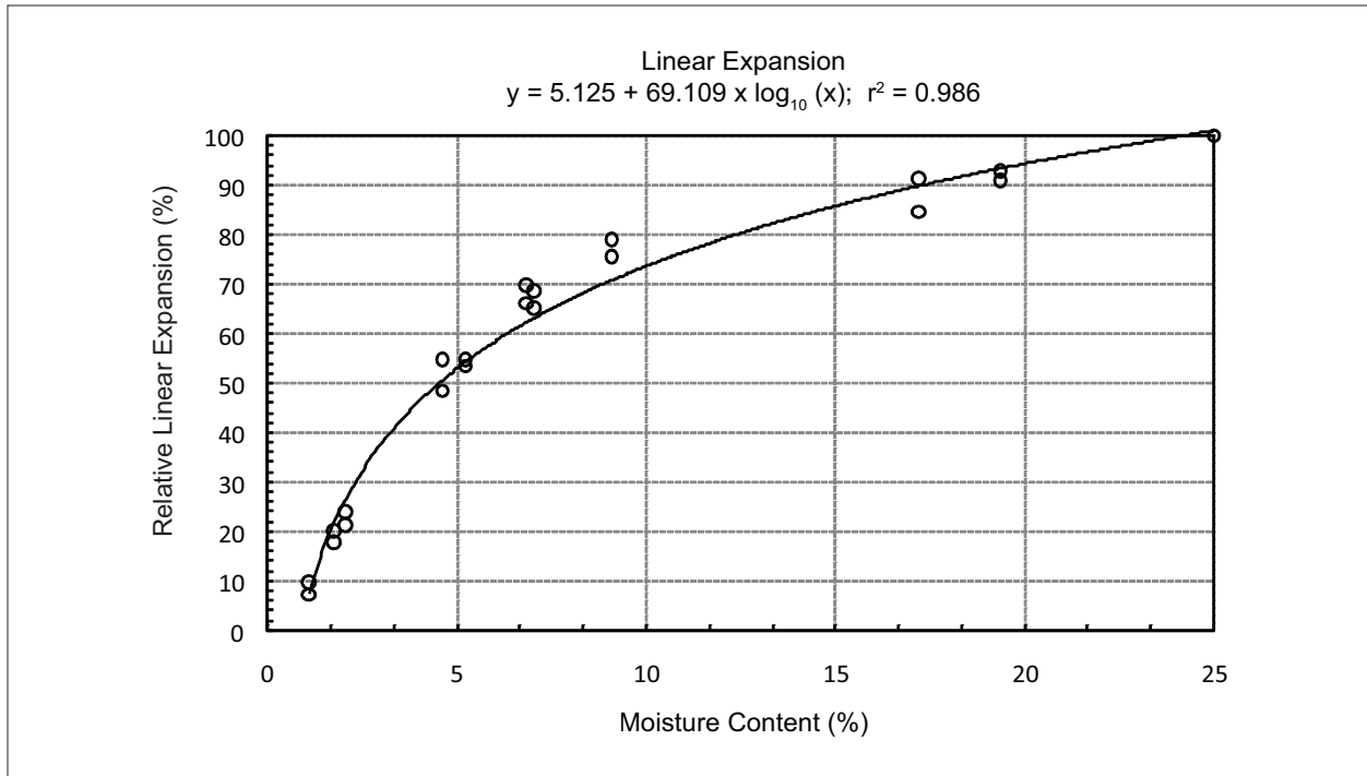
Figure 2. Relative Linear Expansion as a Function of Moisture Content
