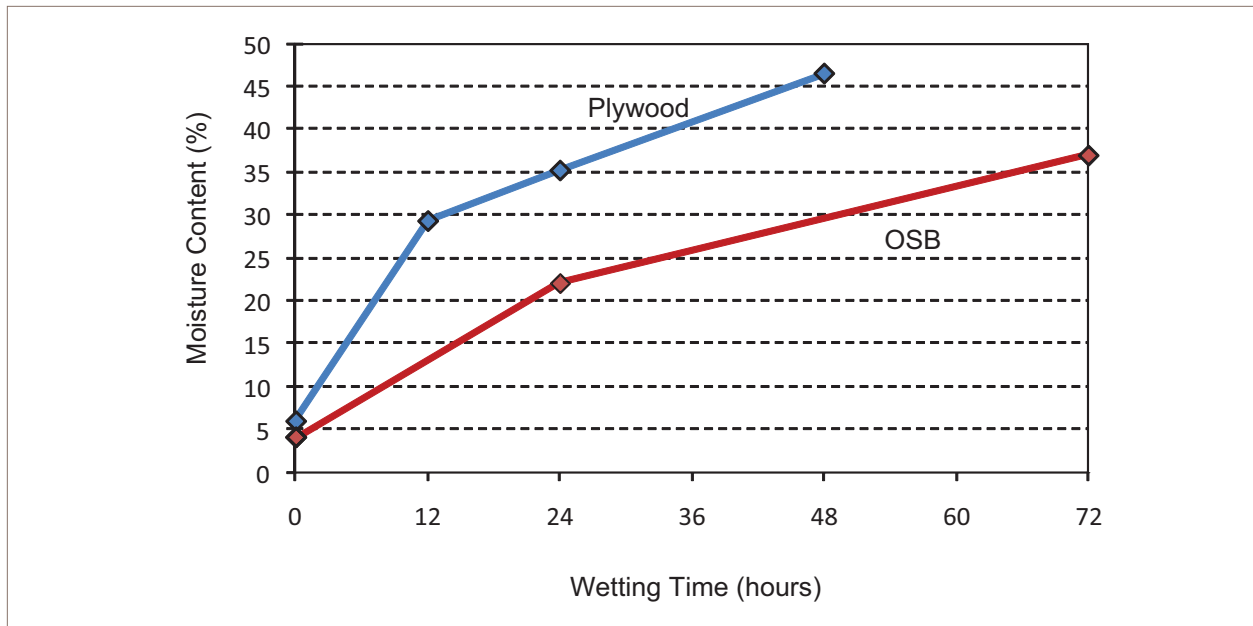
Figure 1. Panel Moisture Content During Wetting
