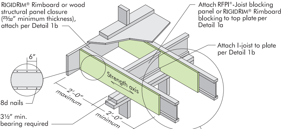
FIGURE 4a RFPI®-JOIST CANTILEVER REINFORCEMENT METHODS (See Figure 4c to determine recommended method)
